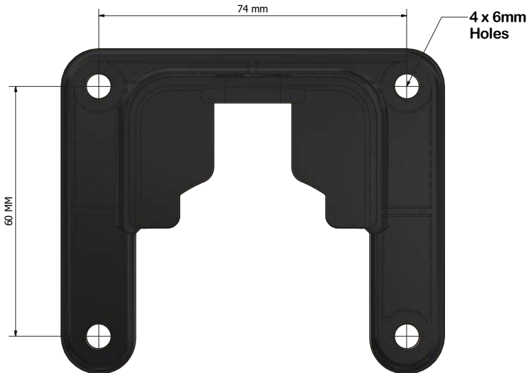
WALL BRACKET DRILL PATTERN 12
